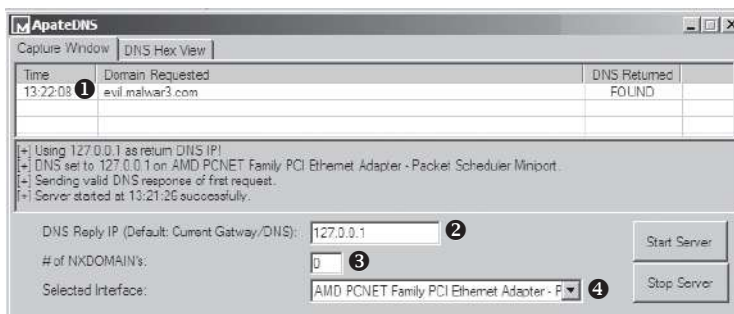
Figure 3-9: ApatеDNS responding to a request for evil.malwar3.com
