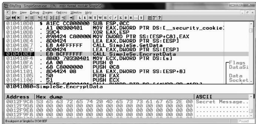
Figure 8-2: Viewing program data prior to the encryption function call
