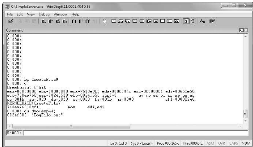
Figure 8-1: Using a breakpoint to see the parameters to a function call. We set a breakpoint on CreateFileW and then examine the first parameter of the stack.
