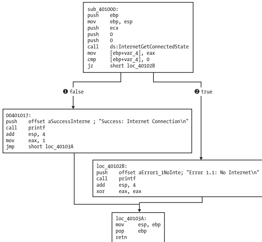
Figure 6-1L: Disassembly flow graph of the function at 0x401000
